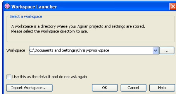
Figure 11 - Workspace Launcher
