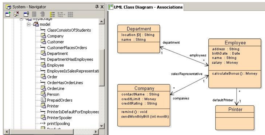
Classes and associations in the navigator
