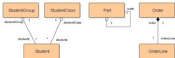
Aggregation versus composition
