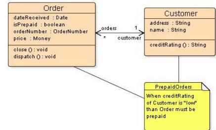
The PrepaidOrders constraint
