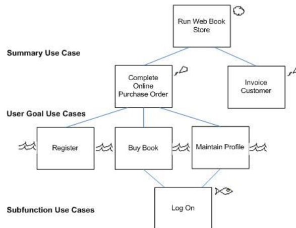
Use cases at different levels
