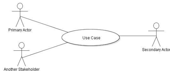
Actors, use cases and communications
